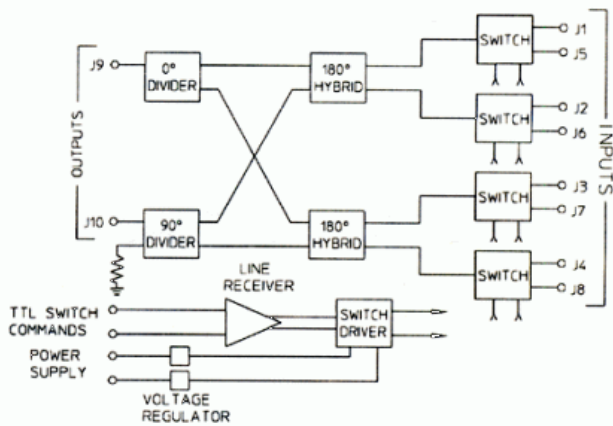
Figure 8: Beamformer Subsystem Schematic
