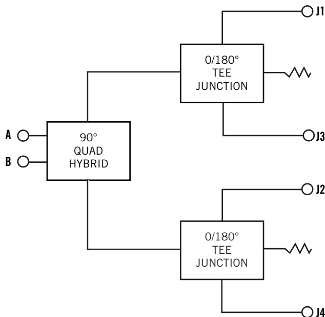
Figure 2: Quadrupole Network Schematic
