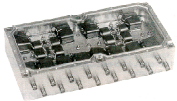
Figure 10: 0.5 to 110 MHz 16 Element Beamformer
