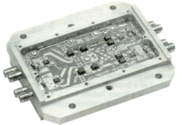
Figure 6: Airborne Warning System Beamformer
