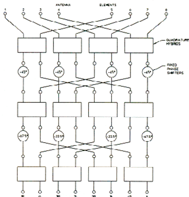
Figure 5: Eight Element Beamforming Matrix
