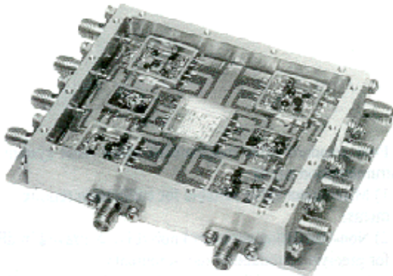
Figure 9: Beamformer Sub-System for Airborne Application
