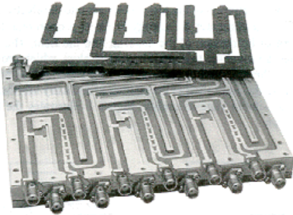
Figure 12: Helicopter Beamformer Application
