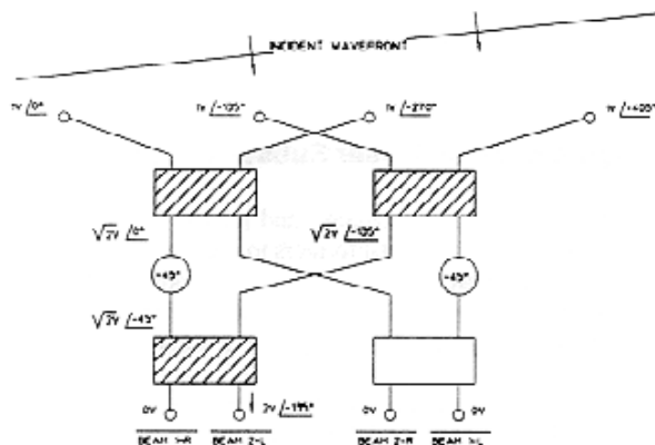
Figure 4: Four Element Beamforming Matrix
