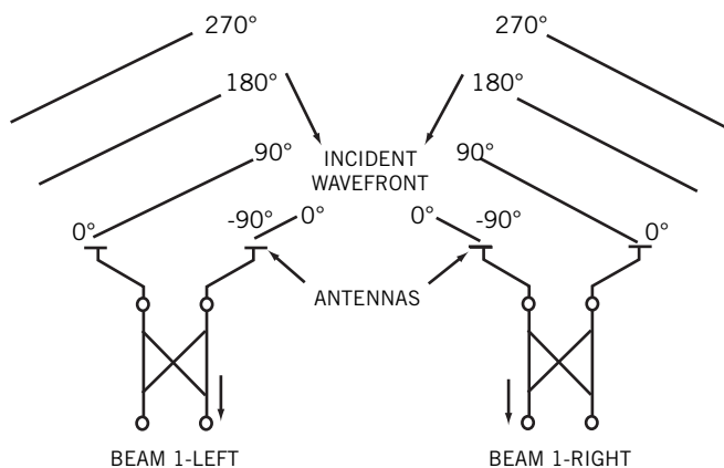
Figure 1: Simple Beamformer Using Quadrature Coupler
